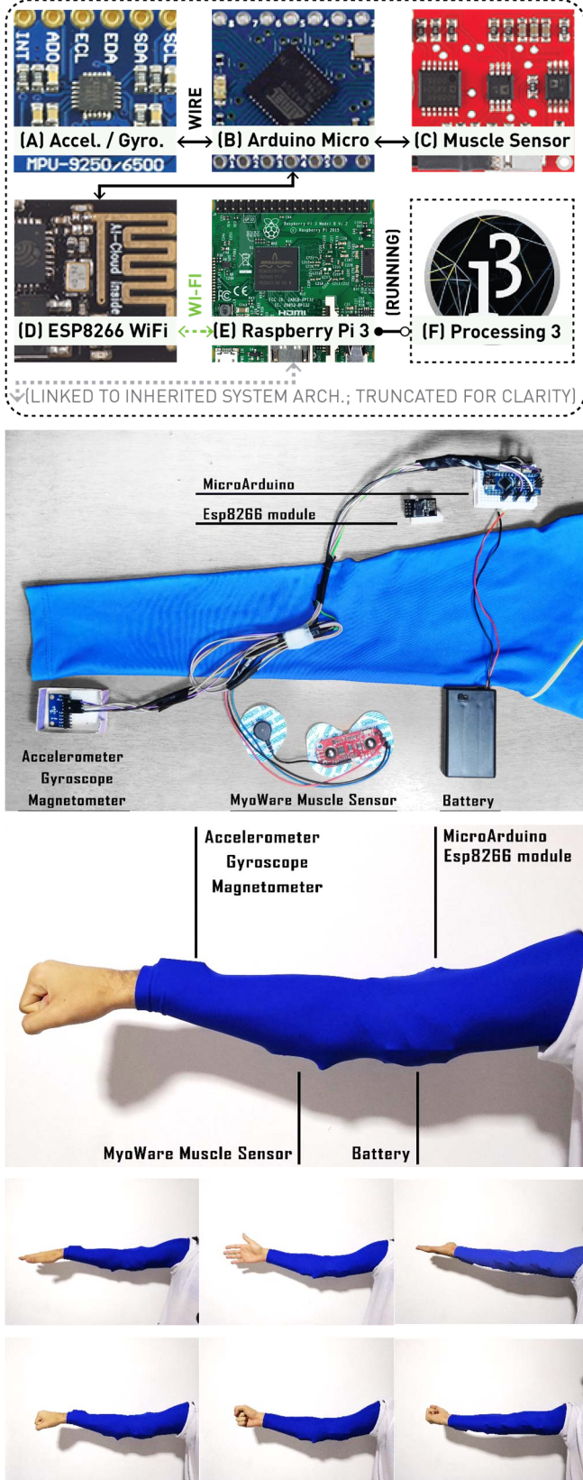
Fig. 1. System diagram and Smart Sleeve description (worn and unworn).
