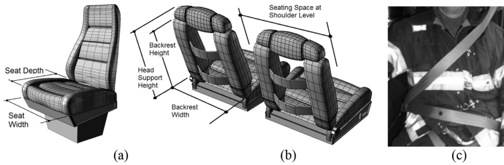
Fig. 1. Seat and seatbelt configurations: (a) seat pan width and depth; (b) backrest width, backrest height, head support height, and unit seating space; and (c) three-point seatbelt (Type II belt), including the shoulder strap and lap belt; the lap belt alone is a Type I belt.
